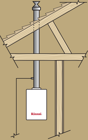
Interior - roof penetration
